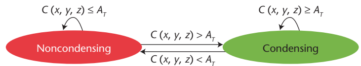
Figure 5. CTM for an avian limb simulation. A noncondensing cell becomes condensing when exposed to an activator concentration C(x, y, z) above a threshold, and a condensing cell becomes noncondensing when exposed to an activator concentration below a threshold.
