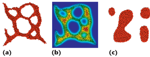
Figure 11. Output of in vitro capillary development simulations. (a) Elongated cells ( L = 30 ) in the absence of cell adhesion, showing the capillary networks found in other research. 9 (b) Chemical concentration from the same simulation, visualizing the field added through Biolog. (c) Vascular islands forming due to the enforcement of rounded cells ( L = 10 ).
