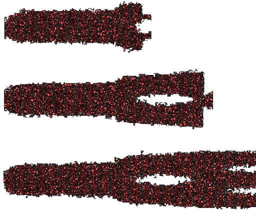
Figure 8. Avian-limb development, visualizing only condensing cells for clarity. The limb forms at the center of a 3D box of cells and is surrounded by mostly noncondensing cells. Formation begins with the humerus after 2,300 Monte Carlo steps (MCSs), followed by the radius and ulna after 3,250 MCS, and finally digits after 4,250 MCS.
